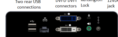
Two rear USB connections DVI-D DVI-I connectors Kensington Lock 12VDC power jack RJ45 Ethernet connector Speaker jack
