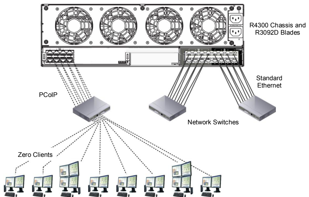
Figure 1. R-Series chassis and R3092D blades connected to zero clients over PCoIP connections
